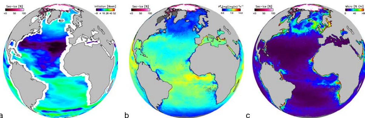
Figure 2: Images of a) phytoplankton phenology (bloom initiation) b) productivity and c) microphytoplankton fraction (courtesy Bob Brewin and Marie Fanny Racault, PML)
